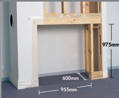
Timber framework, partially plaster board cladded
